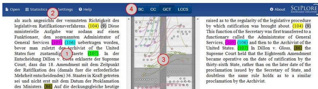
Figure 1: Screenshot of CbPD prototype (left plagiarized translation, right source document)
