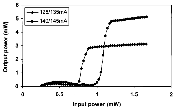
Fig. 2. Measured static decision characteristic for different bias currents to the GCSOAs.
