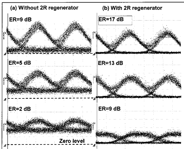
Fig. 4. Eye diagrams with and without the 2R regenerator for signals with different extinction ratios at 2.488 Gb/s. Signal wavelength: 1553.3 nm. ER: Extinction ratio.
