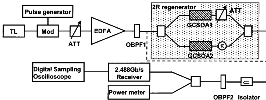
Fig. 1. Experimental setup for 2R regenerator based on a MZI with equal GCSOAs in both arms. TL: Tunable laser. ATT: Attenuator. Mod: Mach-Zehnder modulator. The dashed line indicates the setup without the 2R regenerator.
