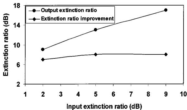
Fig. 5. Output extinction ratio and its improvement as a function of input extinction ratio at 2.488 Gb/s.
