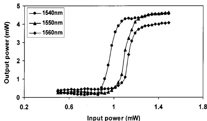
Fig. 3. Regeneration characteristics for different wavelengths, bias currents of two GCSOAs: 135 and 147 mA, respectively.
