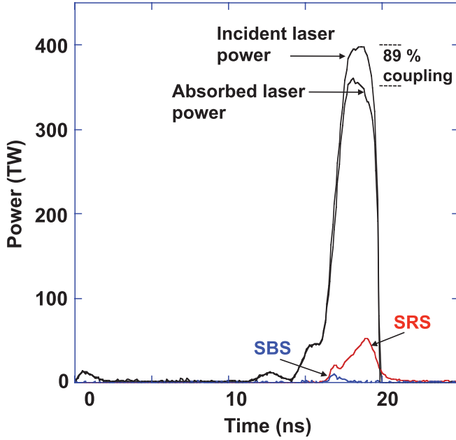
FIG. 2 (color). Measured incident and absorbed laser powers of a 1.22 MJ driven ignition-scale hohlraum shows 89% energy coupling. Also shown are experimental stimulated raman scattering (SRS) and stimulated brillouin scattering (SBS) powers.
