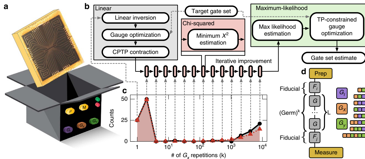
Figure 1 | Gate set tomography is a robust procedure to characterize as-built qubits. (a) GST models the qubit (a single \text{Yb}^+ ion localized in a linear surface electrode ion trap) as a ‘black box’ with a classical interface, and is agnostic to its physical details. (b) Flow chart of GST analysis. Its core is an iterative \chi^2 minimization, over data from increasingly long gate sequences, seeded with a linear inversion estimate. The final step, likelihood maximization, produces an accurate and unbiased estimate of the gate set. (c) A subset of the nearly 5,000 data points taken: observed ‘bright’ counts (black) for sequences of the form G_X^k and the GST estimate’s prediction (red; see Fig. 3). Deviations from ideal gates appear only at k > 1,000 . (d) GST achieves high precision from periodic sequences based on short ‘germs’. Here the 11 germs used for this experiment are shown (coloured boxes), as is the ‘fiducial sandwich’ form of a general GST sequence.
