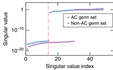
Figure 7 | Sensitivity analysis for germ selection. Here we show the sorted singular values of the Jacobian matrix for different germ sets for the standard \{G_x, G_y, G_z\} gate set. Each singular value of the Jacobian corresponds to a gate set parameter; a large singular value indicates that the chosen germ set provides GST with sensitivity to that parameter. Given that there are always experimentally inaccessible gauge parameters, it is impossible to be sensitive to all parameters. The dashed red line indicates the number of gauge parameters for this gate set (14). The blue triangles are singular values for a Jacobian with the amplificationally complete 11-germ set used for the March 2015 GST runs; all singular values corresponding to non-gauge parameters are large. The purple triangles are singular values for the three-germ set containing just the bare gates G_x, G_y and G_z . It is amplificationally incomplete, as indicated by the presence of near-zero singular values that correspond to non-gauge parameters.
