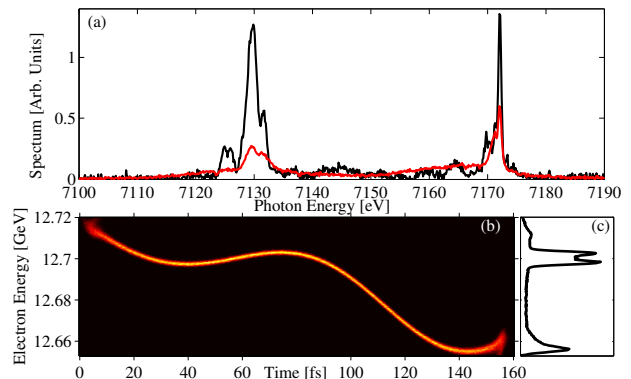
FIG. 5. (a) two-color self-seeded spectrum obtained by using the (-1,1,3) and (1,-1,3) reflections, single-shot (black), average on 100 shots (red). The two color lines are separated by 43 eV ( \sim 0.6\% ) which is wider than the SASE bandwidth for the normal LCLS operation. The pulse energy for the shot was 120 \mu\text{J} . (b) LiTrack simulated phase space obtained by manipulating the X-band linearizer. (c) Simulated two energy levels electron beam energy profile.
