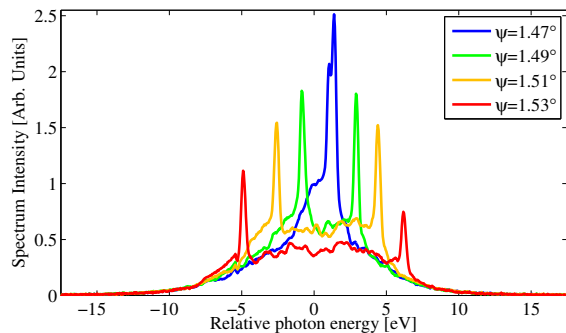
FIG. 3. Average spectra from 111 consecutive shots for single-crystal two-color self-seeded beams with photon energy close to 8.43 keV. The pitch angle was fixed to \theta = 65.28^\circ . (blue) yaw angle \psi = 1.47^\circ . (green) \psi = 1.49^\circ . (orange) \psi = 1.51^\circ . (red) \psi = 1.53^\circ . The used reflection planes were (-1,-3,3) and (-3,-1,3) . The average spectra are shown without post-processing, including the SASE pre-pulse. The plateau between the two narrow colors is mainly due to the wide-bandwidth head part amplified in the second undulator section.
