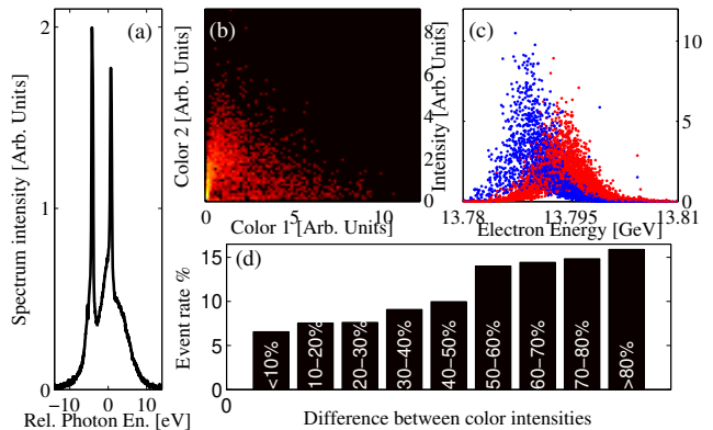
FIG. 4. Single-crystal two-color self seeding experimental results for 3500 consecutive shots. Photon energy was close to 8.43 keV, the reflections used were (2,0,2) and (0,2,2) . (a) Average spectrum. (b) Correlation between the first and second color intensities in a 1 eV bandwidth around each color average peak energy. (c) Single-shot intensities in a 1 eV bandwidth for both colors vs electron beam energy, (blue) color 1; (red) color 2. (d) Histogram of the events rate as function of the difference between the intensities of the two colors.
