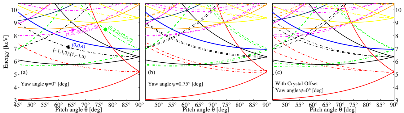
FIG. 2. Photon energy values at which diffraction occurs in a diamond crystal, as a function of the pitch angle \theta for fixed values of yaw angle \psi . Each curve corresponds to reflection from a different set of crystallographic planes. (a) Yaw angle \psi = 0^\circ . Stars represent demonstrated two-color working points. (b) Yaw angle \psi = 0.75^\circ . Different colors represent planes with different h^2 + k^2 + l^2 value. Dash-dotted lines are double-lines (two sets of crystal planes excited) that are superposed for \psi = 0^\circ and can be separated with a non-zero yaw angle. (c) Correcting for the small crystal orientation offset deduced from experimental measurements of the energies as a function of (\theta, \psi) values.
