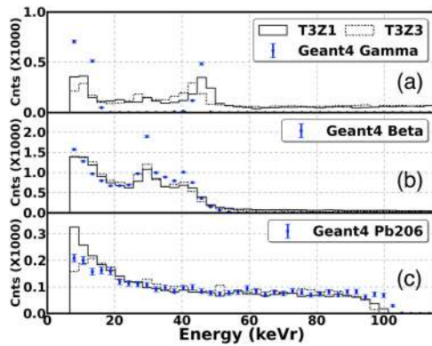
FIG. 4. Comparison of data from the two detectors with a Geant4 simulation. (a) Gamma electron recoil band (data with ionization yield > 0.8 , including the not simulated continuous spectrum from bulk gamma interactions), compared with the simulated X-ray peaks at 12 and 46.5 keV. (b) Beta band (data with yield 0.4–0.8), compared with the simulated beta decays from ^{210}\text{Pb} or ^{210}\text{Po} . (c) ^{206}\text{Pb} recoil band (data with yield < 0.4 ), compared with the simulated ^{206}\text{Pb} recoils from ^{210}\text{Po} decay. Normalizations of the simulations in (a) and (b) were fixed by the normalization needed to match data and simulation in (c). Unlike the perfect simulation classifications, there is significant mixing in the data yield-based classification between “gammas” and “betas,” and between “betas” and “recoils of ^{206}\text{Pb} ” at energies below \sim 20 keV.
