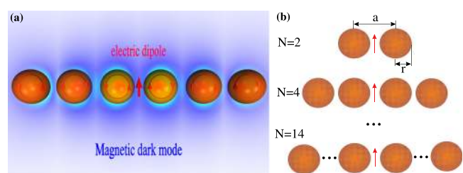
FIG. 1. (a) Excitation of a dark magnetic mode in the chain of dielectric nanoparticles by an electrical dipole emitter. (b) All-dielectric dimer ( N = 2 ), quadrumer ( N = 4 ), and dekatesseramer ( N = 14 ) nanoantennas in the form of chains with the same period a = 200 nm. The dielectric constant of the nanoparticles is \epsilon = 16 ; the radii of nanoparticles are r = 70 nm.
