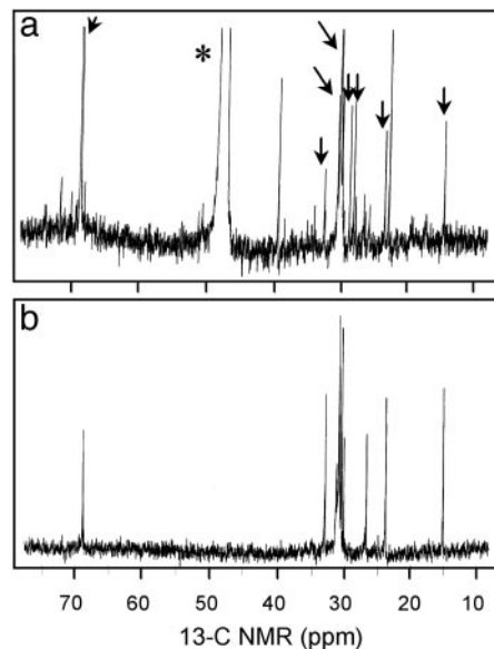
Fig. 4. 13 C NMR spectra of PfTx from Pfiesteria . (a) PfTx from P. shumwayae (CAAE1024C) after size exclusion (HW40F column) and subsequent passage through three sequential C 18 columns using d 4 methanol (*) as a solvent (supporting information). This material, from a fish-fed culture, shows multiple molecular species (congeners) compared with b; arrows indicate peaks in common with b. (b) PfTx from algae-fed P. piscicida (CCMP1832) after the same chromatographic steps used to generate a, followed by passage through a bidentate column using 100% HPLC-grade water as a solvent (supporting information).
