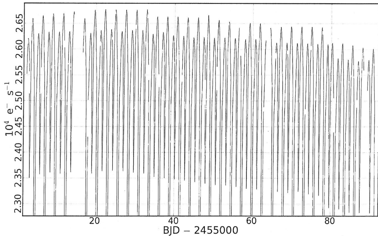
Fig. 1.— Quarter 2 long cadence SAP light curve of the eclipsing binary star V1950 Cyg (KIC 12164751; Horne (2008)), produced by the PyKE tool kepdraw . The most-prominent systematic effect in this light curve is the long-term decay in flux from the target which falls by 3% over the duration of the quarter. This drop is a consequence of differential velocity aberration pushing the under-captured target position across the fixed pixel aperture over time.
