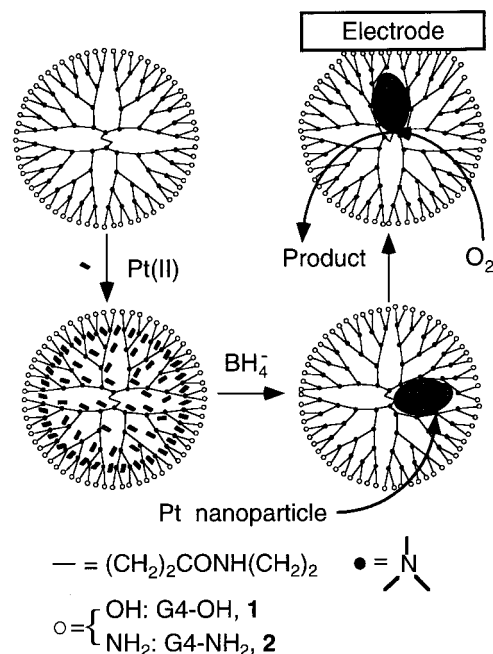
Fig. 1. Schematic illustration of fourth-generation (G4) PAMAM dendrimers having -\text{OH} and \text{NH}_2 terminal groups, synthesis of Pt nanoparticles within the hydroxyl-terminated dendrimer template, and attachment of the composite to an electrode surface. Between 12 and 60 \text{Pt}^{2+} ions can be loaded into a single dendrimer and, upon reduction with \text{BH}_4^- , an entrapped cluster containing the same number of atoms results. The dendrimer-encapsulated Pt nanoparticles are electrocatalytically active.
