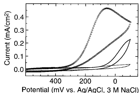
Fig. 4. Cyclic voltammograms of Au electrodes coated with G4-OH in O 2 -saturated 1 M H 2 SO 4 (solid line) or coated with G4-OH(Pt 60 ) in N 2 -saturated 1 M H 2 SO 4 (dashed line) or O 2 -saturated 1 M H 2 SO 4 (circles). Catalytic reduction of O 2 is observed only on the Au/G4-OH(Pt 60 ) electrode. Electrode area: 0.086 cm 2 , scan rate: 50 mV/s.
