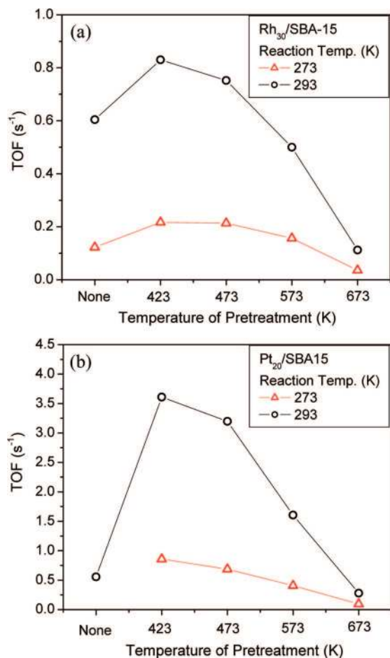
Figure 5. Initial ethylene hydrogenation activity over (a) Rh 30 /SBA-15 and (b) Pt 20 /SBA-15 after reducing in 76 torr of H 2 balanced with He at different temperature. Reaction mixture was 10 torr C 2 H 4 and 100 torr H 2 .
