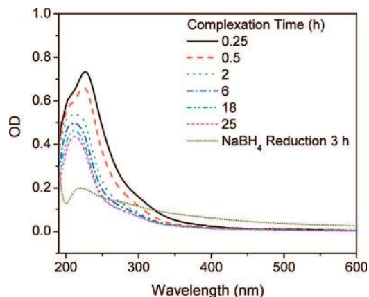
Figure 1. Time-resolved UV-vis spectra of aqueous G4OH(Rh 3+ ) 30 solution and after 3 h reduction by NaBH 4 to yield G4OH(Rh 30 ). The concentration of G4OH is 1.6 μM. The optical path is 1.0 cm. A dendrimer solution of the same concentration is used as the background.
