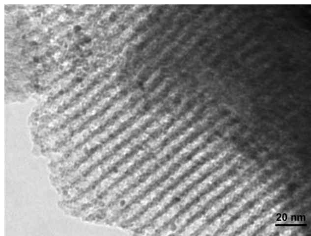
Figure 6. TEM image of the dendrimer encapsulated Rh 30 nanoparticle, after heating in 76 torr of H 2 with He balance at 673 K for 1 h. Many nanoparticles larger than 2 nm are observed because of the sintering of small Rh 30 nanoparticles.
