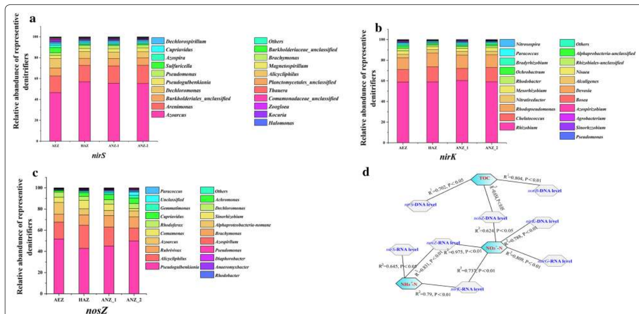
Fig. 4 Community structures in different layers of sediments based on sequence analysis of nirS (a), nirK (b) and nosZ (c). d Pearson correlation matrix between DNA abundance, RNA transcriptional level of denitrification genes and sediment physicochemical factors. AEZ aerobic zone, HAZ hypoxic zone, ANZ-1 up-anoxic zone, ANZ-2 sub-anoxic zone
