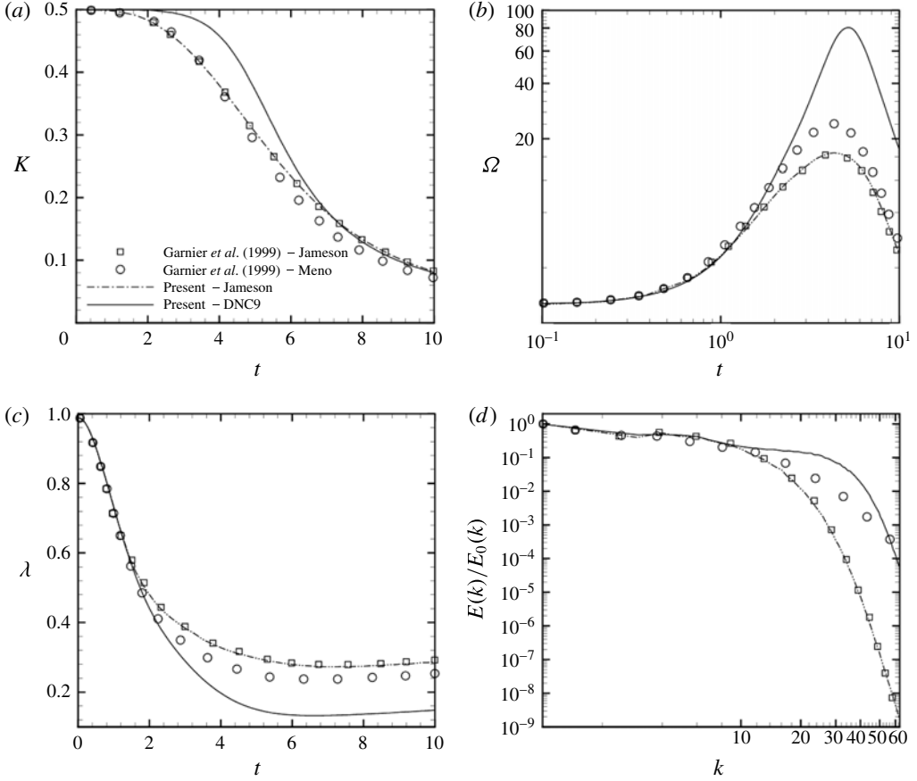
FIGURE 3. Comparison between the present results for CHIT decay at M_{t_0} = 0.2 and \chi_0 = 0 using the ninth-order scheme and Jameson's second-order scheme and those of Garnier et al. (□) based on a fifth-order modified ENO scheme (MENO) and Jameson's scheme. The grid in use is composed by 128^3 cells. Time histories of the turbulent kinetic energy (a), enstrophy (b), pseudo-Taylor microscale (c) and spectrum of the turbulent kinetic energy at t = 10 (d).
