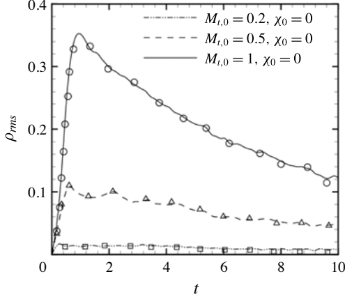
FIGURE 4. Comparison of the present results for a ninth-order accurate scheme with those provided by Garnier et al. (□) using a fourth-order ENO scheme, for different choices of the initial conditions. Lines denote the present results, symbols results from the reference.
