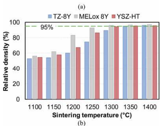
Fig. 5 (a) Density and (b) relative density of the YSZ pellets at different sintering temperatures.
