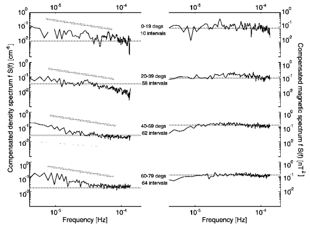
FIG. 2.—Compensated spectra fS(f) from (variance-averaged) spectra of Ulysses data, near solar minimum in several latitude ranges, indicated on the panels, along with the number of intervals in each average. A total of 194 intervals are employed in the analysis. Right: Magnetic spectra. Left: Density spectra. The horizontal bars are reference lines, and a line corresponding to a Kolmogoroff spectrum is also shown. The 1/f range is less evident in density at low latitude.
