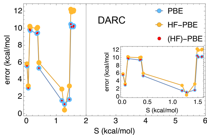
Figure S2: Same as Fig. 2, but for the DARC dataset.
