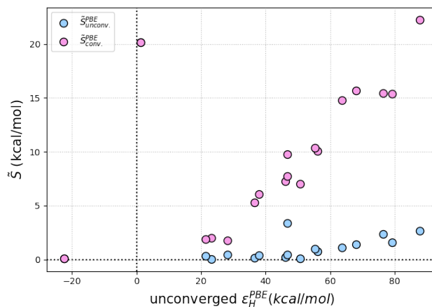
Figure 6: Relationship between unconverged HOMO energy ( \epsilon_H^{PBE} ) of the anion and density sensitivity \tilde{S}^{PBE} for the electron affinities. \epsilon_H^{PBE} energies are mostly positive as calculated from a finite basis set (if a loss of a fraction of an electron is enabled in the calculations \epsilon_H^{PBE} would hit 0). The results are taken from Table 2, and include both converged (HOMO \approx 0.000 a.u.) and unconverged \tilde{S} values.
