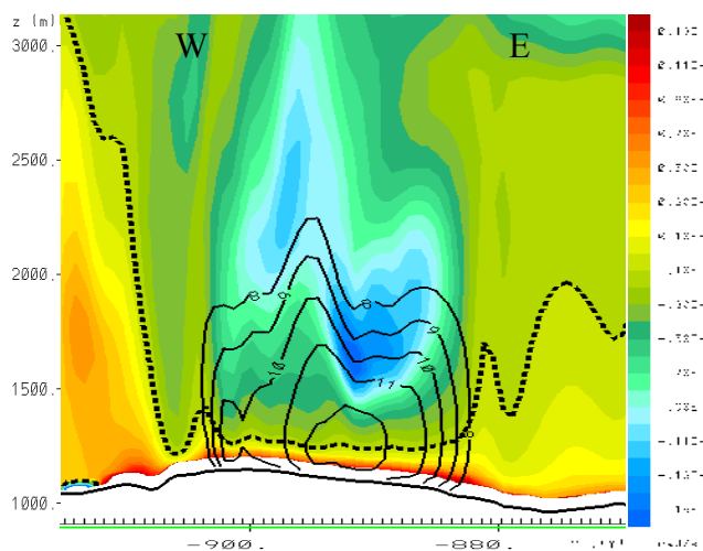
Fig. 7. Wind speed (solid black contours from 8\text{--}12 \text{ m s}^{-1} every 1 \text{ m s}^{-1} ) and \xi relative vorticity component (colour scale) at 12:50 UTC for a WE vertical cross-section at y = -645 \text{ km} . The dashed black line represents \xi = 0 .
