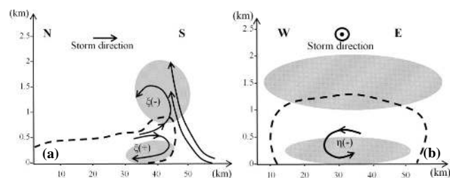
Fig. 10. Schematic representation of the flow structure during the cool pool intrusion. The dashed line indicates the boundary of the density current. Shaded figures indicate areas of increased turbulence. (a) Considering a NS vertical plane parallel to the axis of motion, the flow is rotating clockwise close to the surface ( \xi+ ) and anti-clockwise above ( \xi- ). (b) Considering a WE vertical plane perpendicular to the motion the flow is rotating anti-clockwise ( \eta- ). The storm direction in this figure is towards the reader.
