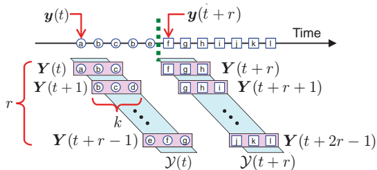
Figure 5: Change-point detection.
