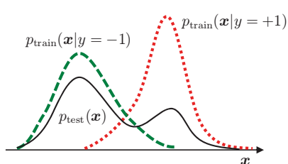
Figure 4: Class-balance estimation.
