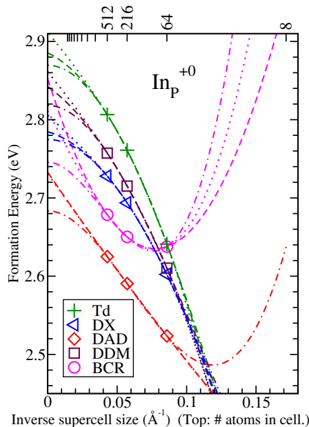
Figure 6. Defect formation energy for \text{In}_\text{P}^{+0} in InP for different structures calculated using only the \Gamma -point. The Td structure has an unbroken tetrahedral symmetry ( T_d ) with breathing mode relaxation only. The DX structure is a C_{3v} symmetry distortion in which the antisite moves towards one of its neighbours (and away from the others). DAD and DDM are both D_{2h} symmetry distortions in which the antisite stays put, but the four neighbours rotate around it in pairs, forming either two dimers or two anti-dimers. In the BCR structure the antisite again shifts off centre, moving towards the middle of one neighbour-neighbour bond (hence in the direction of a bond centre interstitial site). The finite size fittings assume scaling with the powers 1/L+1/L^2 (dashed), 1/L+1/L^3 (dotted) and 1/L^2+1/L^3 (dot-dashed).
