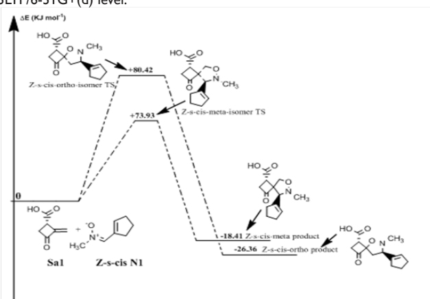
Figure 5 Energetic profile of the reaction of Z-s-cis-isomer N-methyl substituted nitronel with norsarkomycin.
