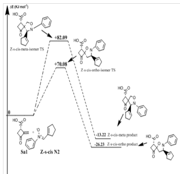
Figure 7 Energetic profile of the reaction of Z-s-cis-isomer N-phenyl substituted nitronel with norsarkomycin.
