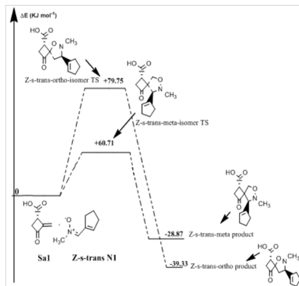
Figure 6 Energetic profile of the reaction of Z-s-trans-isomer N-methyl substituted nitronel with norsarkomycin.
