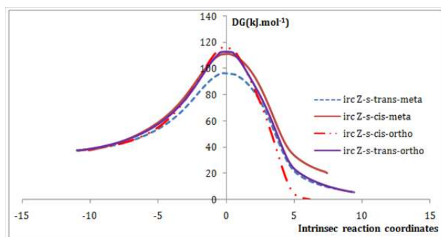
Figure 4 Intrinsic reaction coordinate (IRC) for reactions between Norsarkomycin and different isomers of nitronel IRC performed at the B3LYP/6-31G+(d) level.
