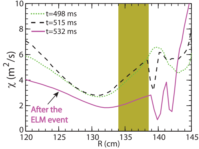
FIG. 6: The plasma effective thermal diffusivity as a function of R for the three MPPTS time points: t = 498 (dotted line), 515 (dashed line) and 532 ms (solid line) with the shaded region denoting the high- k measurement regions as used in Fig. 4 (from about R = 134 to 138.5 cm).
