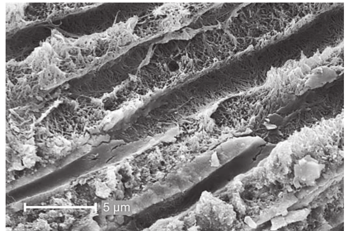
Fig. 7. SEM image of a cross section of a dentine specimen subjected to erosion in hydrochloric acid (pH 1.6; 6 \times 2 min/day, storage in a mineral salt solution; 9 days), then fractured and critical point dried. The tubules are cut longitudinally. Sharp border between the fully demineralised and the fully mineralised tissue.
