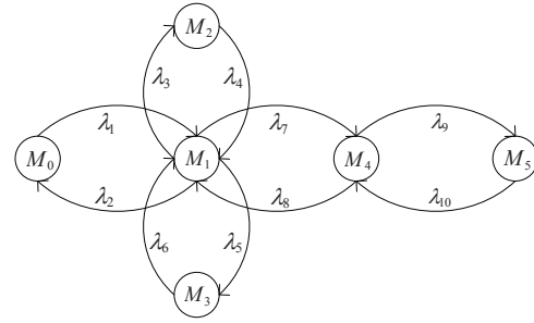
Fig. 6. The equivalent CTMC
