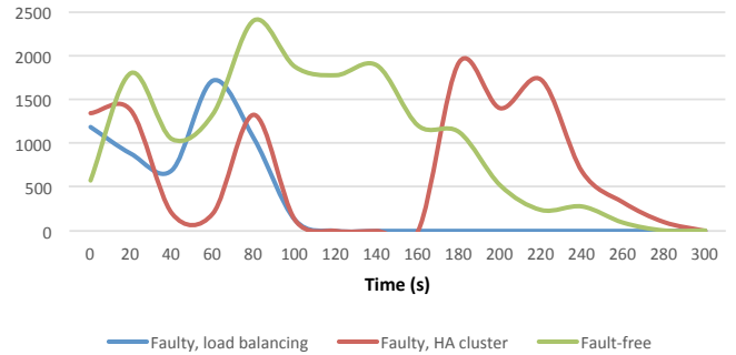
Fig. 10. Network throughput during the injection of a VNF crash.
