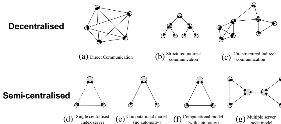
Figure 1 - P2P Architectures
