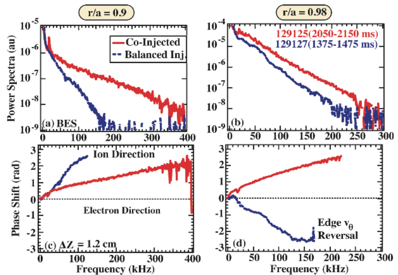
FIG. 5. Cross-power spectra and phase shift of poloidally displaced BES channels ( \Delta Z = 1.2 cm) at r/a=0.9 and r/a=0.98 in co-injection and balanced injection plasmas with the ion VB drift directed away from the X-point illustrating the flow reversal in the later case.
