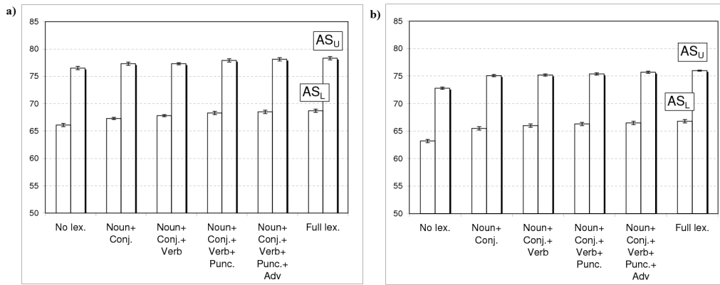
Figure 8 Results for incremental lexicalization for the classifier-based parser a) on Projective HF Treebank , b) on Entire Treebank
