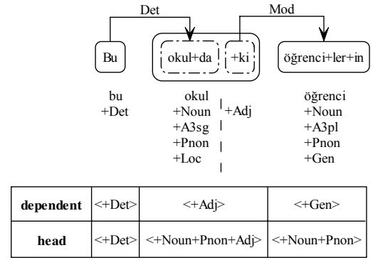
Figure 4 Reduced IG representation for Word-based model #2
