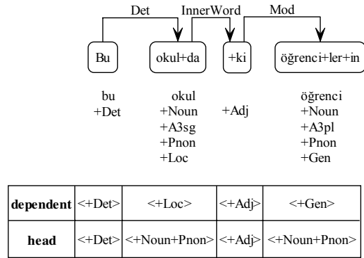
Figure 5 Reduced IG representation for IG-based model
