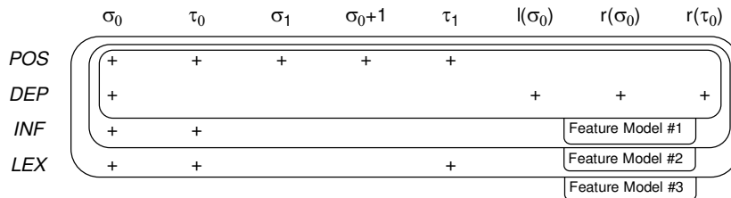
Figure 6 Feature models for the classifier-based parser
