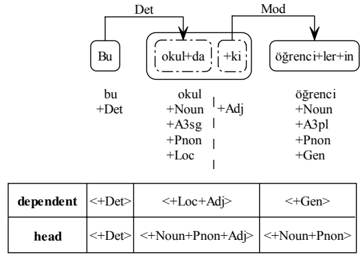
Figure 3 Reduced IG representation for Word-based model #1
