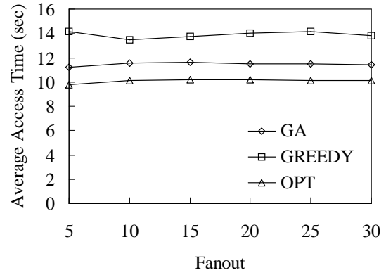
Figure 14: The average access time with the value of fanout varied
