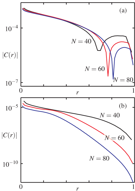
FIG. 11: The NESS density-density correlations |C(r)| across the chain as a function of the fraction distance r about the centre for \Delta = 2 and f = 0.1 . In (a) a moderate dephasing \gamma = 0.05 was included. The correlations are long-ranged and extend over a larger fraction when increasing N . This evidenced by the kink, coming from C(r) changing sign, moving to larger r . In (b) a strong dephasing \gamma = 1 was present and the correlations are short-ranged as shown by their diminishing size and extent with increasing N .
