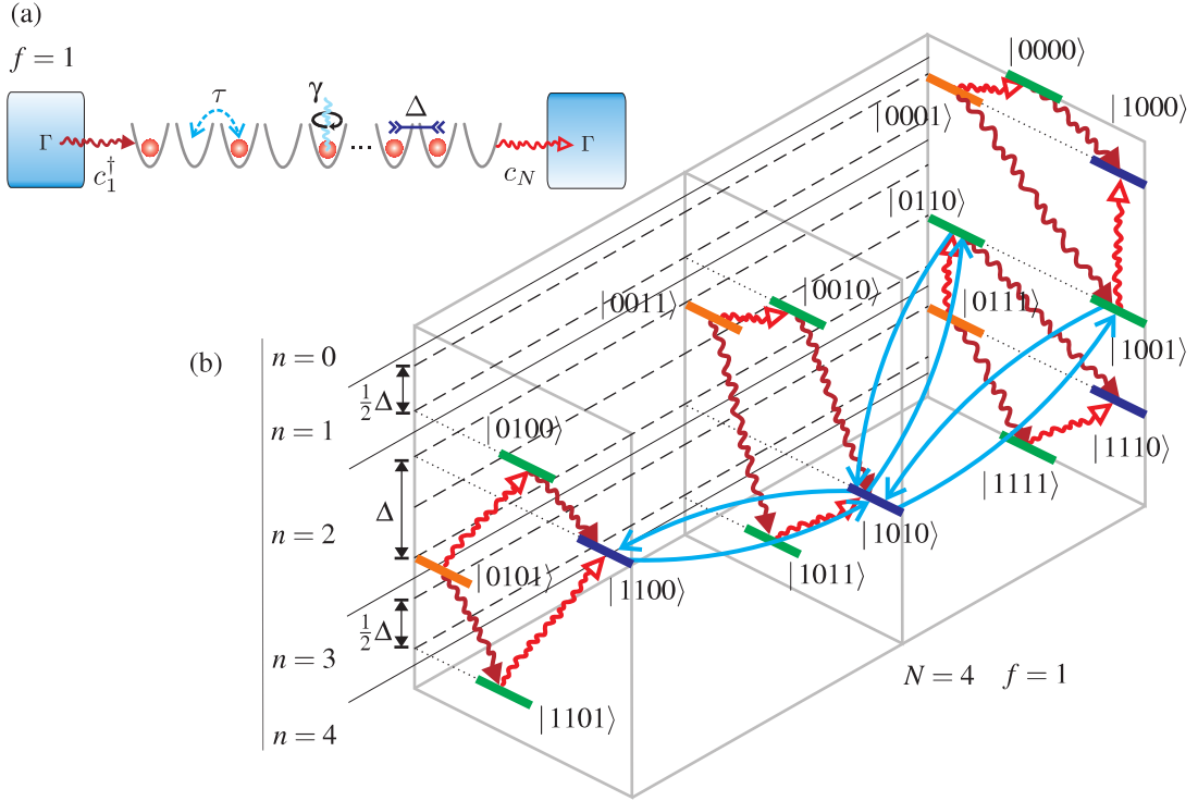
FIG. 14: (a) A schematic of the system, showing the coherent hopping \tau , the nearest-neighbour density-density interaction \Delta , dephasing \gamma , and the incoherent boundary driving in the strong driving limit f = 1 where the bias is maximal. In this case the driving incoherently pumps particles into the system at site 1 and ejects them at site N , both at a rate \Gamma . (b) For N = 4 sites and f = 1 the complete set of driving quadruplets and the transitions induced by coherent hopping between them from the half-filled domain state |1100\rangle is shown. The vertical axis displays the particle number sectors and energy gaps between configurations. We observe that for N = 4 one hop connects |1100\rangle to |1010\rangle , which is a dark configuration of its quadruplet, and a further hop is needed before it is coherently connected to a configuration that is not dark to the f = 1 driving. This disconnection between the half-filled domain configuration and the driving only occurs for N \geq 4 , and so this is the smallest size which displays NDC.
