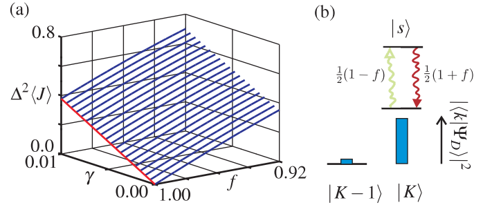
FIG. 17: (a) The NESS current \langle J \rangle , rescaled by \Delta^2 , for K = 20 is shown as a function of the driving f and dephasing \gamma zoomed in around the limit f = 1 , \gamma = 0 insulating point (see Fig. 8(a)). The behaviour at f = 1 with \gamma is emphasized by the additional (red) line. (b) In the strong driving limit f \sim 1 , the \Lambda_R^- process |K\rangle \rightarrow |s\rangle occurs at a rate \propto (1-f) \ll 1 making it slow (as indicated by being faded out), while the \Lambda_R^+ process |s\rangle \rightarrow |K\rangle occurs at a rate \propto f \approx 1 and so is rapid. The dominant driving process is therefore |K\rangle \rightarrow |s\rangle \rightarrow |K\rangle , which has the effect of destroying any coherence |K\rangle has with other states, such as |K-1\rangle .
