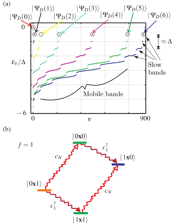
FIG. 6: (a) The energy eigenspectrum of the spinless fermion Hamiltonian governing the chain for N=12 and \Delta=10 . Energies \epsilon_\nu have been shifted by \frac{1}{4}\Delta(N-1) so that the state |\Psi_D(0)\rangle = |00\cdots 00\rangle has zero energy. The spectrum includes contributions from all particle number sectors n=0, \dots, 12 ; since the spectra arising from n=0, \dots, 5 are identical to those of n=7, \dots, 12 , only the former are shown in addition to n=6 . The highest lying eigenstate for each sector |\Psi_D(n)\rangle is highlighted and seen to be isolated by a gap of O(\Delta) from eigenstates composed of break-away configurations (states with the outermost particle of the domain breaking away, or a hole propagating through the domain). The braces give an indication of the location of mobile and flattened bands for n=6 . (b) For any f the driving alone incoherently connects a quadruplet of configurations |0\mathbf{x}0\rangle, |0\mathbf{x}1\rangle, |1\mathbf{x}0\rangle, |1\mathbf{x}1\rangle . The situation for f=1 is shown where the driving can be seen to only pump into the so-called dark configuration |1\mathbf{x}0\rangle .
