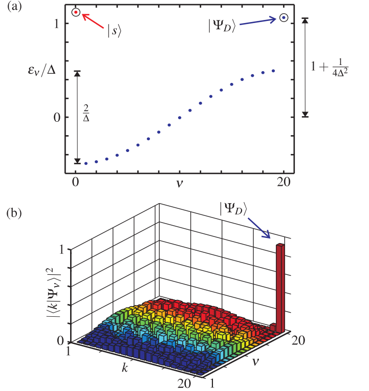
FIG. 9: (a) The spectrum \varepsilon_v of the Hamiltonian for the toy model for K = 20 and \Delta = 2 . Eigenstate v = 0 is the highlighted auxiliary state |s\rangle whose energy has been set arbitrarily. The highest-lying eigenstate v = K is also highlighted and is the approximate dark-state of the model |\Psi_D\rangle . Beneath this state, separated by a gap O(|\Delta|) , is a band of eigenstates |\Psi_v\rangle split by the small hopping. (b) The probability distributions |\langle k|\Psi_v\rangle|^2 of the eigenstates over the configurations |k\rangle are shown. The band of eigenstates are seen to be delocalized over the configurations |1\rangle, |2\rangle, \dots, |K-1\rangle and expunged from the boundary configuration |K\rangle , while the characteristic of a bound state |\Psi_D\rangle is predominately peaked at |K\rangle with exponential tail into the bulk.
