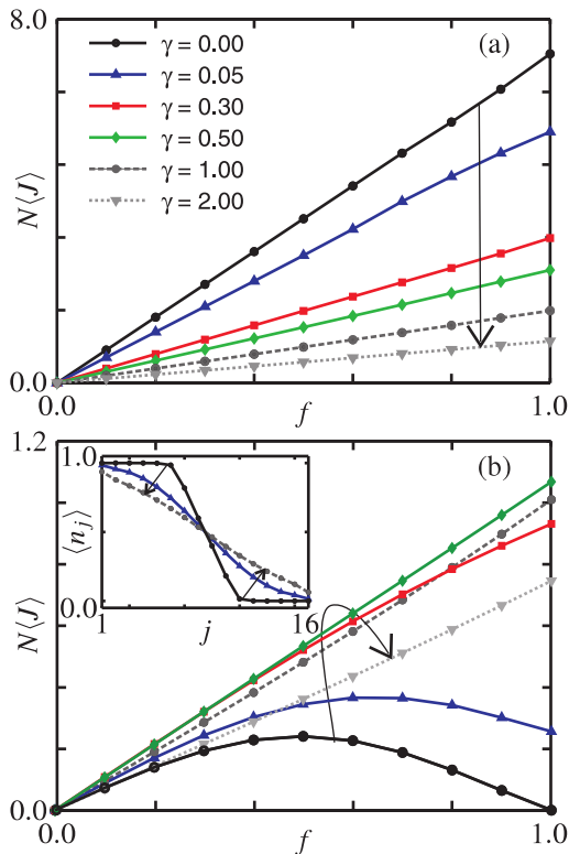
FIG. 2: (a) The current-driving profiles in the weakly-interacting regime \Delta = 0.5 for increasing (as indicated by the arrow) dephasing rates \gamma and N = 16 . (b) Identical plot to (a) but in the strongly-interacting regime \Delta = 2 . Inset. The density \langle n_j \rangle of the system when \Delta = 2 , f = 1 , and N = 16 , corresponding to \gamma = 0, 0.05, 1.00 .
