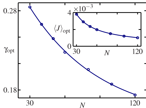
FIG. 5: Optimal dephasing \gamma_{\text{opt}} for different sizes of the system, at f = 0.1 , \Delta = 2 and \Gamma = 1 (circles). The solid line corresponds to the exponential decay \gamma_{\text{opt}} = \gamma_{\text{opt}}^{\text{TL}} + a \exp(-N/b) , with a = 0.252 , b = 85.9 and \gamma_{\text{opt}}^{\text{TL}} = 0.109 . Inset: Optimal current \langle J \rangle_{\text{opt}} as a function of N . The solid line corresponds to the power law decay \langle J \rangle_{\text{opt}} = aN^{-b} , with a = 0.0948 and b = 0.94 ; as N \rightarrow \infty , \langle J \rangle_{\text{opt}} \rightarrow 0 .
