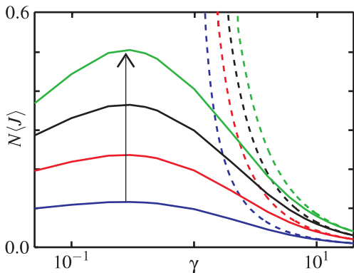
FIG. 4: The current as a function of \gamma for driving biases f = 0.1, 0.2, 0.3 and 0.4 (from bottom to top curve) with \Delta = 2 , and N = 40 . The dashed lines correspond to \langle J \rangle_{\Delta=0} the non-interacting analytic result 53,56 .
