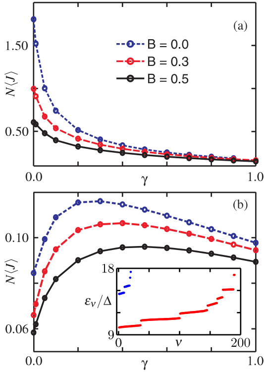
FIG. 13: The current through the system for several staggered potential strengths B , for N = 40 , f = 0.1 and \Gamma = 1 , with (a) \Delta = 0.5 and (b) \Delta = 2.0 . Inset. Energy eigen-spectrum for one (blue) and two (red) excitations of a chain of N = 20 , with staggered potential B = 2 and interaction \Delta = 10 .
