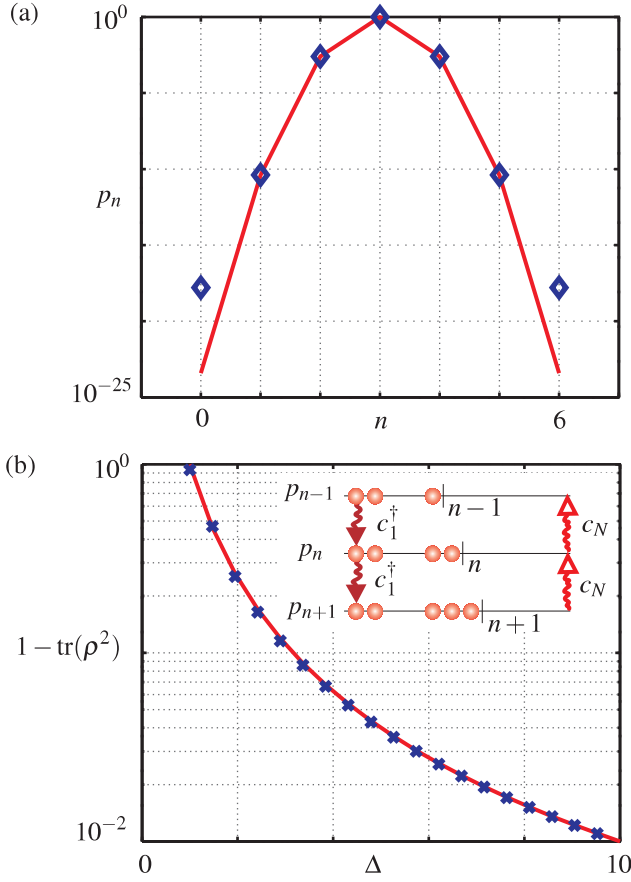
FIG. 16: (a) The probability p_n on a logarithmic scale of the NESS \rho occupying the n particle sector is shown for an exact calculation ( \diamond ) for N = 6 and \Delta = 10 , and the predicted form (solid line) given in Eq. (A4). (b) The purity 1 - \text{tr}(\rho^2) against \Delta of the NESS \rho on a logarithmic scale for an exact calculation ( \times ) for N = 6 and the predicted form (solid line) given in Eq. (A5). The inset shows a schematic of the detailed balance approximation applied to compute these predictions.
