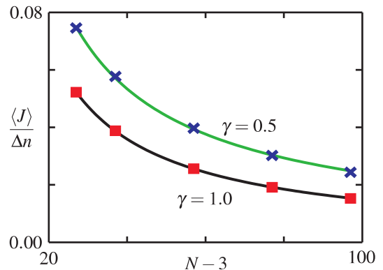
FIG. 3: The current \langle J \rangle at f = 1 , divided by the resulting density difference \Delta n between the ends of the system (excluding the boundary), is plotted against the system size N - 3 up to N = 100 sites. The data is for dephasing rates \gamma = 0.5 (x) and \gamma = 1.0 (■). The solid lines show the fitting to \langle J \rangle / \Delta n = \kappa (N - 3)^{-\alpha} for each \gamma . These yield \kappa = 1.288 and \alpha = 0.863 for \gamma = 0.5 , and \kappa = 1.228 and \alpha = 0.958 for \gamma = 1.0 .
