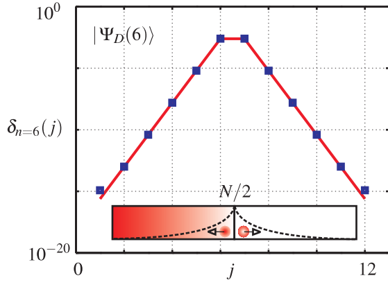
FIG. 15: For the eigenstate |\Psi_D(6)\rangle for N = 12 and \Delta = 10 the exact density deviation \delta_n(j) from the corresponding boundary domain configuration |B_n\rangle is shown (■), along with \delta_n^{\text{ph}}(j) predicted by considering single particle/hole propagation (solid line). The inset shows a schematic of the expected exponential localization of the domain wall.
