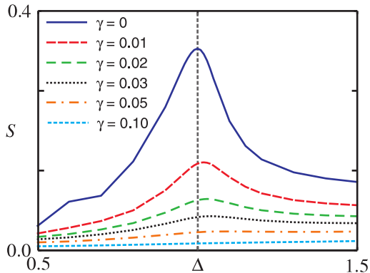
FIG. 12: The half-chain entropy S as a function of \Delta for different \gamma 's, f = 0.1 and N = 40 . The Schmidt coefficients \lambda_\alpha were normalized so the largest coefficient \lambda_1 = 1 .
