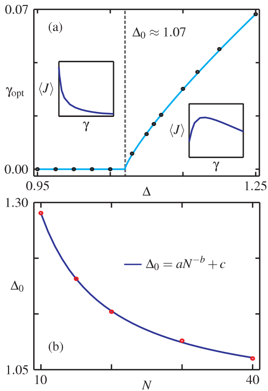
FIG. 10: (a) The optimal dephasing rate \gamma_{\text{opt}} as a function of \Delta , for N = 40 , f = 0.1 and \Gamma = 1 . The circles indicate TEBD results, and the solid line corresponds to the fitted function \gamma_{\text{opt}} \propto (\Delta - \Delta_0)^\beta , with \beta = 0.819 and \Delta_0 = 1.07 . The inset plots show the generic behaviour of \langle J \rangle with \gamma above and below \Delta_0 . (b) The scaling of \Delta_0 with N for f = 0.1 and \Gamma = 1 , along with the fitted power-law shown, where a = 3.906 , b = 1.066 and c = 0.995 .
