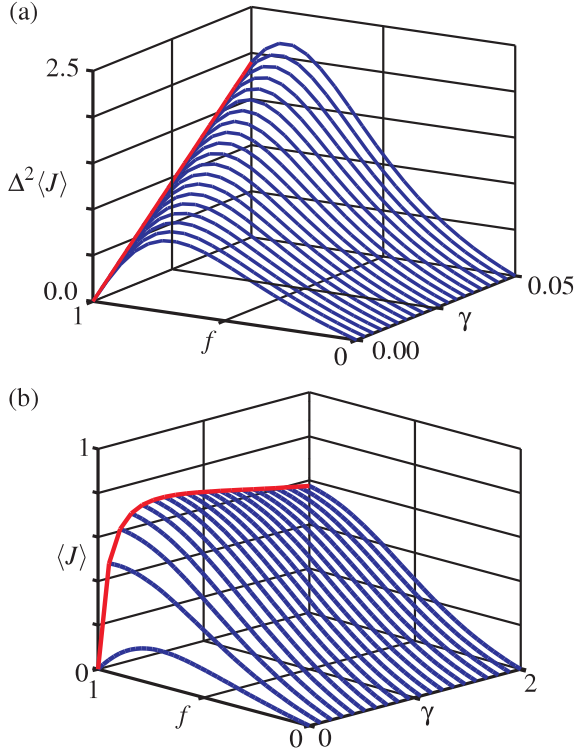
FIG. 8: (a) The NESS current \langle J \rangle , rescaled by \Delta^2 , for K = 20 , as a function of the driving f and dephasing \gamma , described by the approximation in Eq. (14). The behaviour at f = 1 with \gamma is emphasized by the additional (red) line. (b) The exact current-driving profiles of the toy-model as a function of \gamma with \Delta = 2 and K = 20 .
