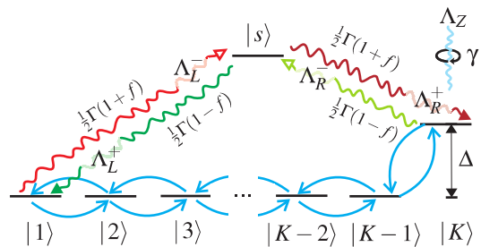
FIG. 7: The schematic of the toy model and its various processes and properties. These include the nearest-neighbour coherent hopping between the set of states |1\rangle, |2\rangle, \dots, |K\rangle , an energy offset \Delta for state |K\rangle , incoherent transitions |1\rangle \leftrightarrow |s\rangle and |K\rangle \leftrightarrow |s\rangle between the boundary states and the auxiliary state |s\rangle , and dephasing at a rate \gamma . The rates for the incoherent driving transitions \frac{1}{2}\Gamma(1 \pm f) are also listed.
