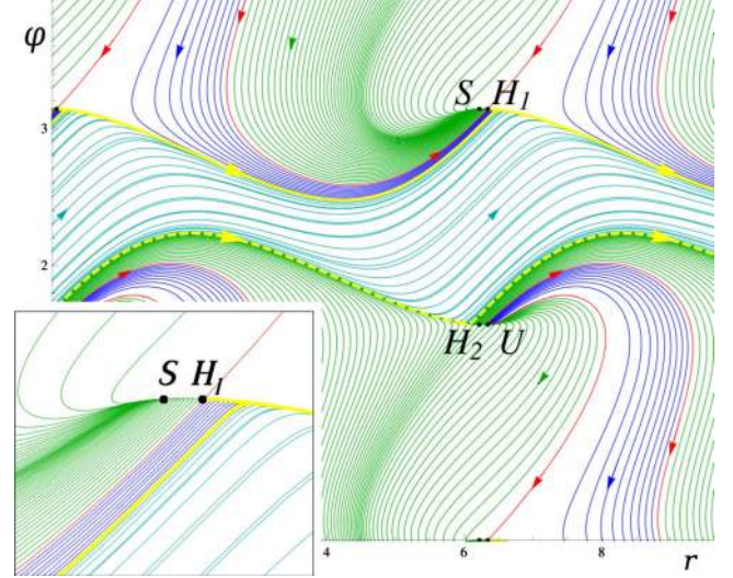
FIG. 2. (Color online) Phase-space trajectories (r, \varphi) for f in the bistable regime ( f_c^* < f < f_c ). S , U , and H_{1,2} are the fixed points. Blue and turquoise trajectories converge to the attracting limit cycle (yellow). Those in green end at the stable fixed point S . Separatrices (red) mark the boundaries between the corresponding regions. The repulsive limit cycle (dashed yellow) is also a separatrix.
