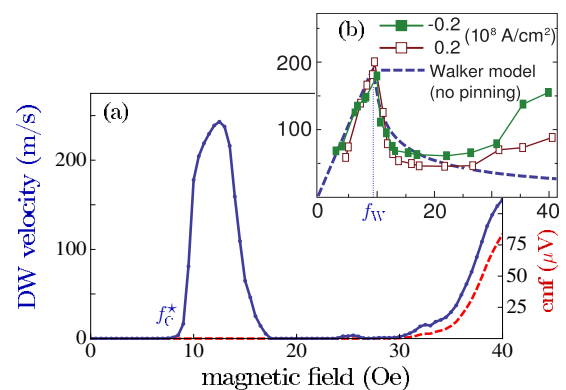
FIG. 1. (Color online) (a) Finite temperature ( T=300 K), zero current force-velocity curves (blue, solid) and emf \frac{\hbar}{e}\langle\dot{\varphi}\rangle (red, dashed) for a DW with pinning, obtained from the numerical solution of Eqs. (2) and (3). Parameters correspond to experiments shown in (b) (see text). Adapted from Ref. 13, the data (b, squares) are for small but opposite currents. In the absence of pinning (Walker model, b, dashed blue line) there is no second rapid increase in v manifest in the data.
