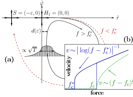
FIG. 3. (Color online) (a) Sketch of the phase space for the coordinates (\tilde{r}, \tilde{\varphi}) , and homoclinic bifurcation. For f < f_c^* (red, dashed), trajectories all end at S . For f > f_c^* (black, solid), the line starting from the unstable direction of H_1 converges to the limit cycle. At T > 0 , the random evolution has Gaussian probability distribution of variance \propto \sqrt{T} . (b) The two types of depinning behaviors at T=0 . For large K_\perp (green, dotted) depinning occurs with \beta = \frac{1}{2} . For intermediate K_\perp (blue, solid) there is a bistable regime of force ( f_c^* < f < f_c ) with a zero-velocity branch and a nonzero one in 1/\log .
