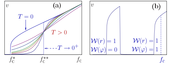
FIG. 4. (Color online) (a) For any finite T there exists a critical field f_c^{**} such that for f < f_c^{**} the albeit small probability of falling into the trap S exceeds that of escape and the velocity is small while the inverse is true for f > f_c^{**} . The curves approach the vertical line as T \rightarrow 0 and all curves cross at f = f_c^{**} to first order in T . (b) For smaller K_\perp (and T=0 ), successive bistable transitions occur, indexed by the winding numbers \mathcal{W}(r) and \mathcal{W}(\varphi) of r and \varphi on one period.
