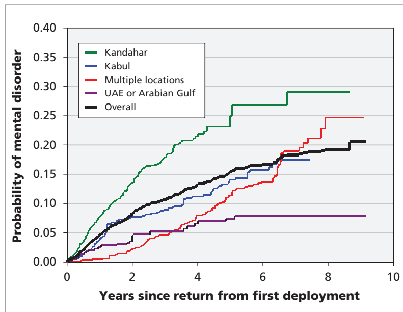
Figure 1: Kaplan-Meier estimates of the probability of a mental disorder attributed to the Afghanistan mission being diagnosed since return from the first deployment, by deployment location. United Arab Emirates (UAE) and Arabian Gulf locations were combined for ease of interpretation because there was no significant difference in incidence density or hazard ratios for these locations in the univariable analyses.
