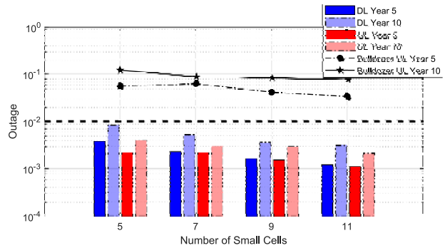
(b) 10 MHz (700 MHz) + 10 MHz (2.6 GHz)
