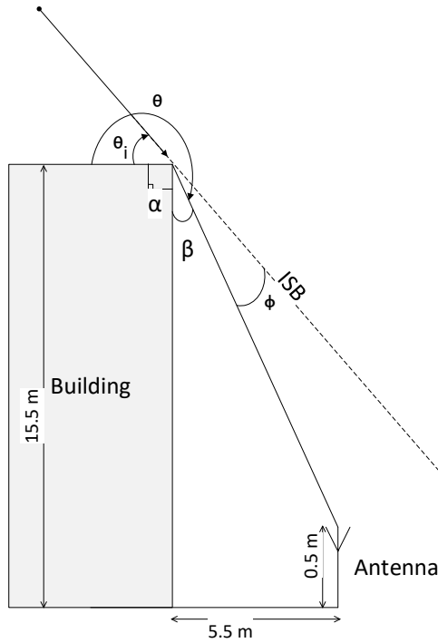
Fig. 1. Side view of the right angle wedge diffraction scenario
