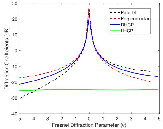
Fig. 4. Depolarization due to diffraction
