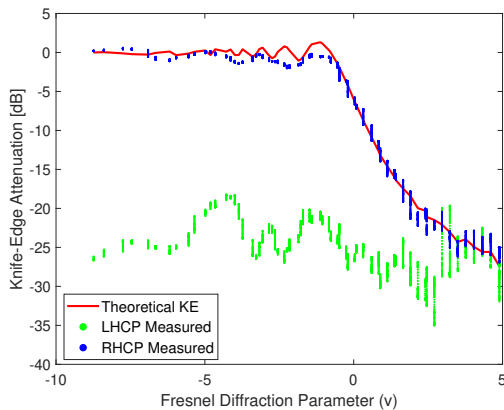
Fig. 3. Path loss vs diffraction parameter
