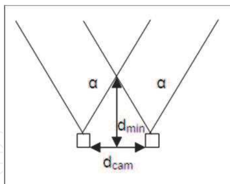
Figure 13. Minimum distance measurable in terms of the cone view angle \alpha and the distance between sensors d_{cam} .
