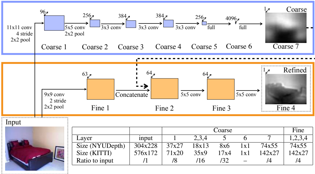
Figure 1: Model architecture.
