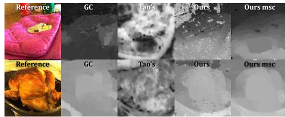
Figure 13. Disparity result comparison between GC, Tao’s, ours and our multi-scale optimization method.
