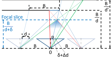
Figure 6. Retrieving the radiances from the center view that correspond to the radiances in other views. In rendering the focal slice shifted from the true disparity d by \delta , the green (red) ray in the center view corresponds to the green (red) ray in the left (right) view. See text for corresponding ray identification.
