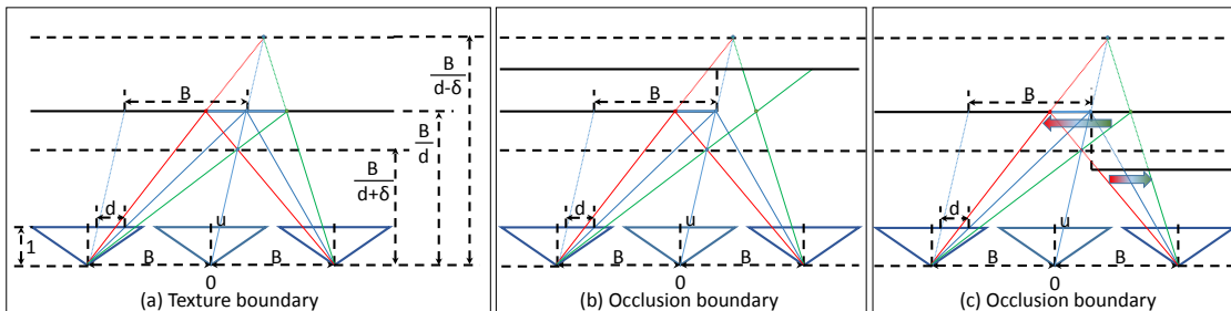
Figure 4. Local symmetry/asymmetry property analysis in LF focal stack.
