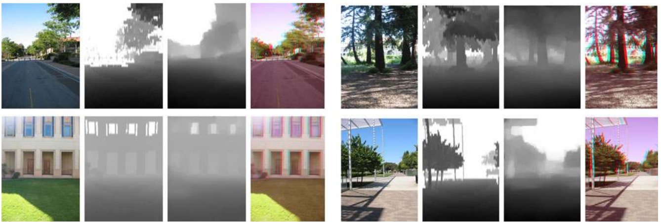
Fig. 8. Single image results obtained on test images from the Make3D data set. Each result contains the following four images (from left to right): original photograph, ground truth depth from the data set, our inferred depth, and our synthesized anaglyph image. The depth images are shown in log scale. Darker pixels indicate nearby objects (black is roughly 1m away) and lighter pixels indicate objects farther away (white is roughly 80 m away). Each pair of ground truth and inferred depths are displayed at the same scale.
