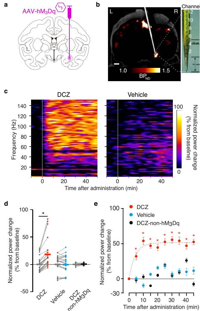
Fig. 5 | DCZ rapidly drives activation of hM 3 Dq-expressing neuronal population in monkey. a , Illustration representing viral vector (AAV2-CMV-hM 3 Dq) injection into one side of the amygdala. b , Coronal PET image overlaying CT image demonstrated that recording contacts on a multichannel electrode (shown on right) were located in an hM 3 Dq-expressing region, which was visualized as a high [ 11 C]DCZ binding site. The high binding observed in the dorsomedial surface corresponds to a site of biological reaction within the recording chamber. Scale bar represents 5 mm. c , Representative LFP activity changes after DCZ (left) and vehicle administration (right). d , Normalized gamma (40 Hz) power change (mean ± sem from baseline) in 10-20 min after intravenous administration of reagents. Data were obtained from hM 3 Dq-positive region (DCZ and vehicle; n = 27 and 26 channels, respectively, acquired across 4 sessions) and non-hM 3 Dq expressing sites (DCZ-non-hM 3 Dq; n = 11 channels, acquired within 1 session). Gray bars indicate baseline. Asterisk represents significant difference from baseline. DCZ t(26) = 7.3 , p = 8.7 \times 10^{-8} ; vehicle t(25) = 0.28 , p = 0.78 ; DCZ-non-hM 3 Dq t(10) = 0.46 , p = 0.65 . e , Plots represent normalized power change (mean ± sem from baseline) as a function of time from vehicle or DCZ administration. Curve represents exponential fit to the data. Asterisks represent significant difference ( p < 0.01 , one-way ANOVA with post-hoc Dunnett) from baseline. Data were obtained from one animal.
