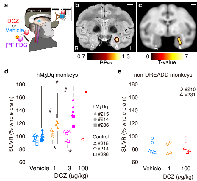
Fig. 6 | DCZ selectively induces metabolic changes in \text{hM}_3\text{Dq} -expressing region in a dose-dependent manner. a , Illustration representing DREADD activation imaging with [^{18}\text{F}]\text{FDG} . Following administration of DCZ at effective doses, [^{18}\text{F}]\text{FDG} was injected and PET scan was performed to assess DREADD-induced brain metabolic change. b , Coronal PET image overlaying MR image representing specific [^{11}\text{C}]\text{DCZ} binding ( \text{BP}_{\text{ND}} ) in a monkey (#215). Filled and open arrowheads indicate the \text{hM}_3\text{Dq} -expressing and control region in the amygdala, respectively. Scale bar represents 5 mm. c , Brain areas with significantly increased [^{18}\text{F}]\text{FDG} uptake after DCZ injection (3 \mu\text{g}/\text{kg} , n=6 scans) compared with vehicle ( n=6 ) overlay on MRI template (uncorrected p < 0.001 , repeated measures one-way ANOVA, monkeys #215 and #236). Significance level is given as a t-value represented on a color scale. d , Relationship between the dose of DCZ administration and standardized FDG uptake (SUVR) in monkeys expressing \text{hM}_3\text{Dq} in the amygdala. Filled and open symbols are the values at \text{hM}_3\text{Dq} -expressing amygdala and contralateral control region, respectively. * p < 0.01 , paired t-test (for 1 \mu\text{g}/\text{kg} DCZ, t(3) = 6.0 , p = 0.009 ; for 3 \mu\text{g}/\text{kg} DCZ, t(5) = 9.7 , p = 2.0 \times 10^{-4} ). # p < 0.05 , one-way ANOVA with post-hoc Tukey test ( F(2,14) = 25.06 , p = 2.4 \times 10^{-5} ; vehicle vs. 1 \mu\text{g}/\text{kg} , p = 0.013 ; vehicle vs. 3 \mu\text{g}/\text{kg} , p = 0.03 ). e , Same as d , but for amygdala of control monkeys without \text{hM}_3\text{Dq} -vector injection (non-DREADD monkeys; #210 and #231). There was no significant dose effect (one-way ANOVA, F(2,12) = 2.29 , p = 0.14 ).
