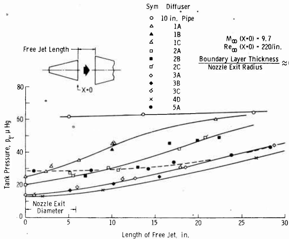
Fig. 13 Diffuser Performance with Clear Jet
