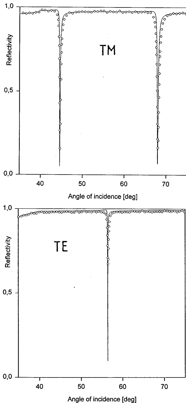
FIG. 7. TE and TM waveguide modes of a poled polymer (polymethacrylate with azobenzene side chains) with corresponding model fit used for retrieving the anisotropic refractive index and layer thickness.
