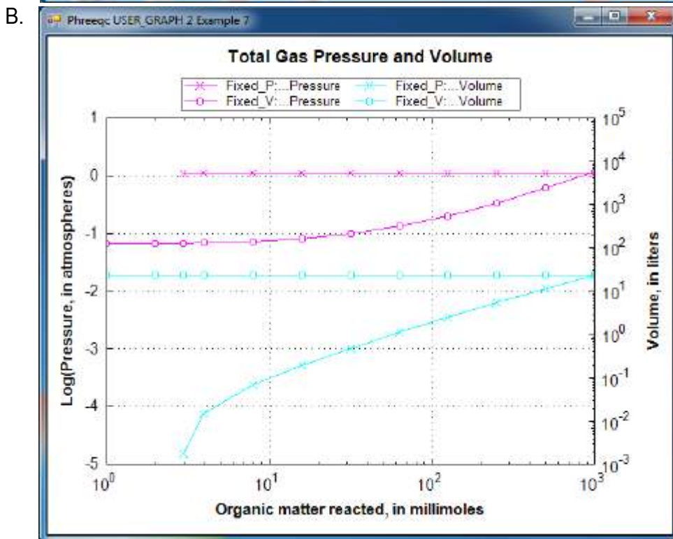
Figure 8. (A) Compositions and (B) total gas pressures and volumes of a fixed-pressure and a fixed-volume gas phase during decomposition of \text{CH}_2\text{O}(\text{NH}_3)_{0.07} (organic matter) in water. (The partial pressure of ammonia gas is less than 10^{-7} atmospheres throughout and is not shown.)
