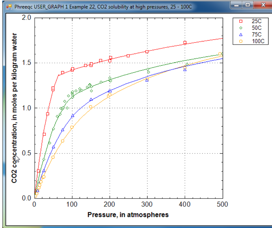
Figure 27. Solubility of CO 2 gas as a function of gas pressure at 25, 50, 75 and 100 °C. Data points are from compilations by Duan and others (2006) and Spycher and others (2003); lines are calculated with PHREEQC.
