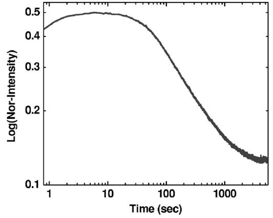
FIG. 3. \log_{10} - \log_{10} plot of the fluorescence time trace of a collection of bare CdSe QDs excited at 514 nm with an excitation intensity flux of 15 \text{ kW/cm}^2 . The first absorption peak of the QD/hexane solution was at 592 nm and the diluted solution was spin coated on a bare glass substrate.
