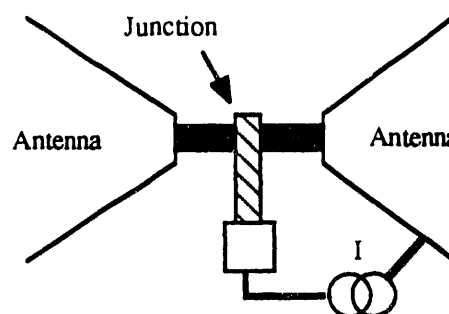
Fig. 1. Schematic of the radiation coupling and temperature readout configuration. The rf current from the superconducting antenna is dissipated in the resistive metal strip (black strip), the resulting temperature rise of the electrons in the strip are measured as a change in the voltage across the junction which is biased at a constant current I . The contact to the superconducting electrode is made of a superconductor whose T_c is much higher than that of the electrode.
