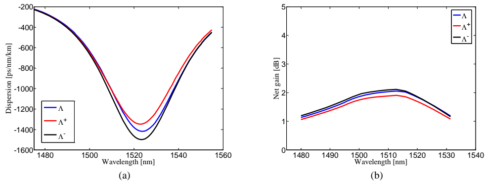
Fig. 7. (a) Dispersion and (b) net gain characteristics of the optimized PCF with a tolerance of \pm 1\% in the lattice constant. Red and black color solid lines represent the variation of lattice constant by \pm 1\% , while blue color solid line stands for the optimized PCF structure.
