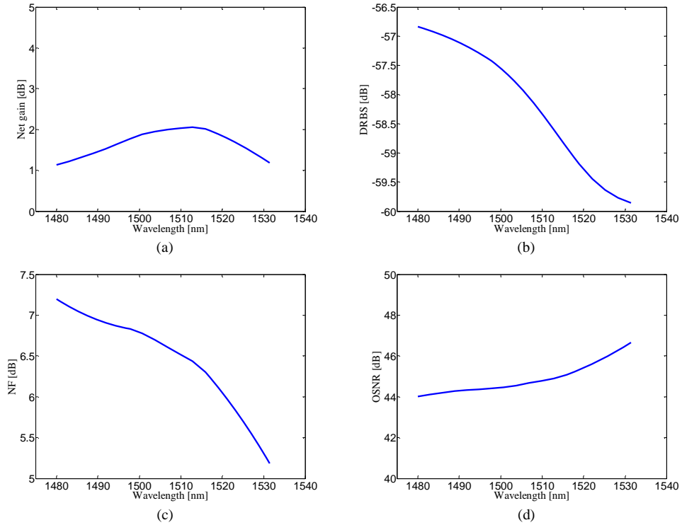
Fig. 5. Spectral variation of (a) net gain, (b) DRBS, (c) noise figure, and (d) optical signal-to-noise ratio for a single pump of 1450-nm and 18 S-band channels with an initial power of -10 dBm/ch in 1.45-km long optimized PCF.
