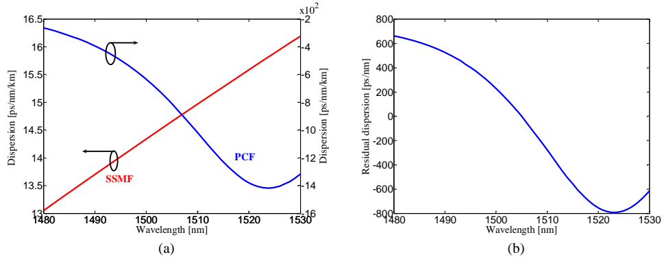
Fig. 4. (a) Chromatic dispersion of the optimized PCF structure and SSMF. The dispersion for PCF lies between -264 ps/nm/km and -1410 ps/nm/km and (b) Residual dispersion after compensation of dispersion in one span (80-km) of SSMF link by 1.45-km long optimized PCF. The residual dispersion is \pm 700 ps/nm, thus enabling the proposed PCF to be a suitable for 10 Gb/s transmission networks.
