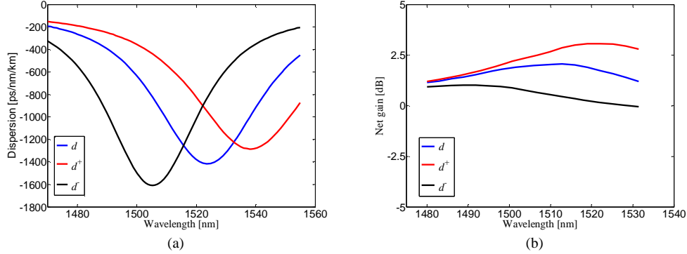
Fig. 10. (a) Dispersion and (b) net gain characteristics of the optimized PCF with a tolerance of \pm 1\% in the hole-diameter d of the 7th and 8th air-hole rings while keeping other design parameters fixed. Red and black color solid curves represent the variation of hole-diameter d of the 7th and 8th air-hole rings by \pm 1\% , while blue color solid curve stands for the optimized PCF structure.
