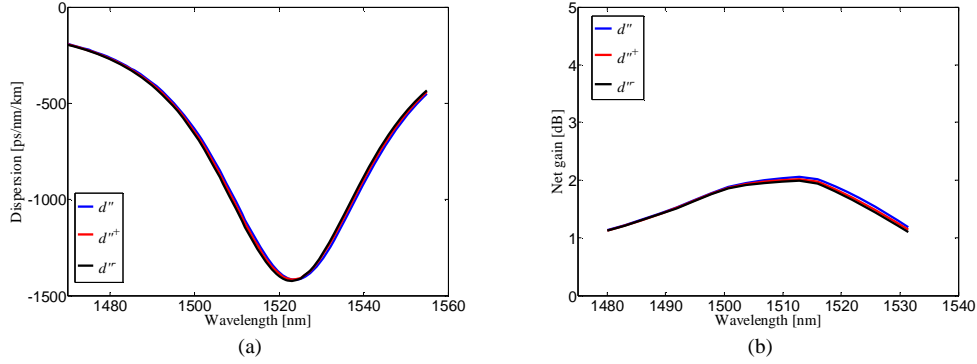
Fig. 11. (a) Dispersion and (b) net gain characteristics of the optimized PCF with a tolerance of \pm 1\% in the hole-diameter d'' of 9-13th air-hole rings while keeping other design parameters fixed. Red and black color solid curves represent the variation of hole-diameter d'' of 9-13th air-hole rings by \pm 1\% , while blue color solid curve stands for the optimized PCF structure.
