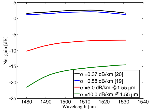
Fig. 6. Variation of net gain as a function of wavelength with fiber attenuation as a parameter.
