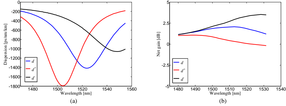
Fig. 8. (a) Dispersion and (b) net gain characteristics of the optimized PCF with a tolerance of \pm 1\% in the hole-diameter d of first five air-hole rings while keeping other design parameters fixed. Red and black color solid lines represent the variation of hole-diameter d of first five air-hole rings by \pm 1\% , while blue color solid line stands for the optimized PCF structure.
