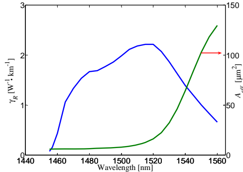
Fig. 3. Variation of RGE and effective area as a function of the wavelength. The RGE is obtained for an unpolarized light source at 1455-nm wavelength. The peak RGE value is 2.21 W^{-1}.km^{-1} at 1.52 \mu m .
