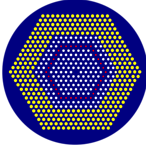
Fig. 1. Transverse cross-section of the optimized PCF structure having lattice constant \Lambda=1.375 \mu\text{m} , d/\Lambda = 0.4434 (1-5th and 7-8th air-hole rings, shown by white color filled circles), d'/\Lambda = 0.2962 (6th air-hole ring, shown by red color filled circles), and d''/\Lambda = 0.60 (9-13th air-hole rings, shown by yellow color filled circles).
