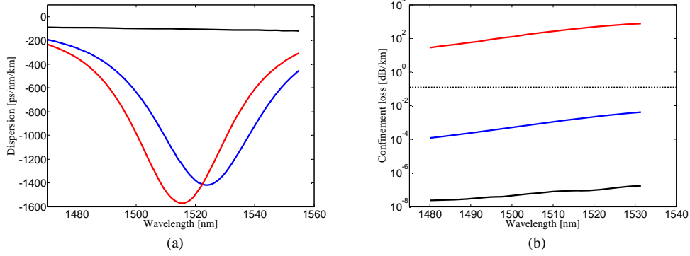
Fig. 2. (a) Chromatic dispersion and (b) confinement loss of three different designed PCF structures; blue curve represents for the optimized fiber design as shown in Fig. 1, red curve denotes the case when the air-hole diameter of air-hole rings from 7 to 13 is d , while black curve stands for the case when the hole-diameter of air-hole rings 7-13 is d'' .
