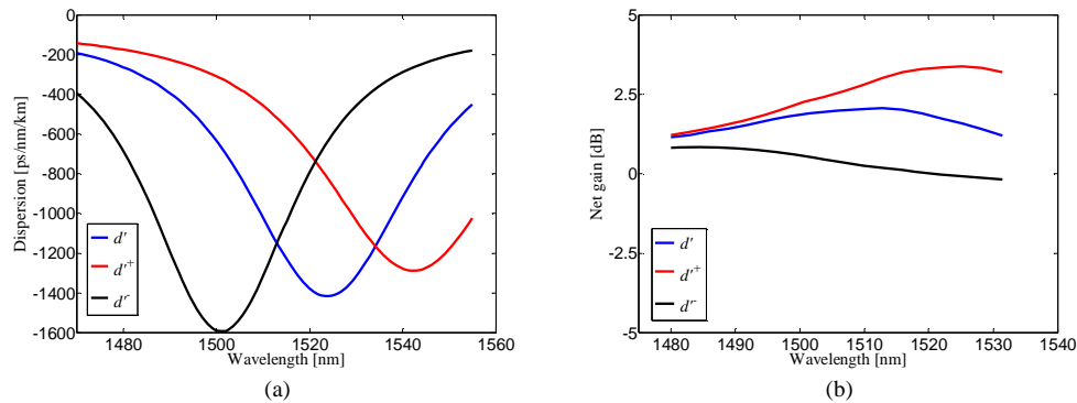
Fig. 9. (a) Dispersion and (b) net gain characteristics of the optimized PCF with a tolerance of \pm 1\% in the hole-diameter d' of ring-core (i.e. 6th air-hole ring) while keeping other design parameters fixed. Red and black color solid curves represent the variation of hole-diameter d' of ring-core by \pm 1\% , while blue color solid curve stands for the optimized PCF structure.
