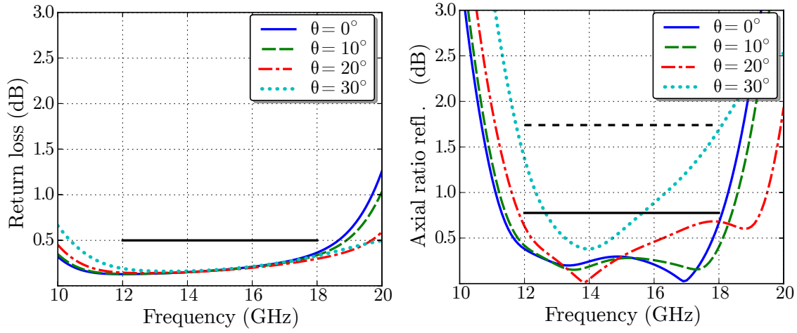
Figure 12: Simulation results of the multilayer CPSS at different angles of incidence, in the plane \varphi = 225^\circ . In the left plot is the LHCP RL, and in the right plot is the AR of the corresponding reflected signal. The solid black lines are the design requirements defined in [4], and the dashed black lines are relaxed requirements of AR < 1.74 dB.
