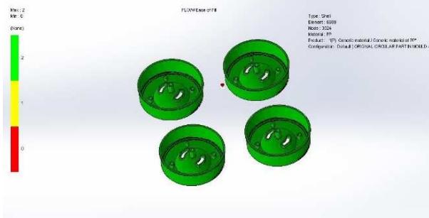
Figure No.7 Analysis of Ease of Fill
