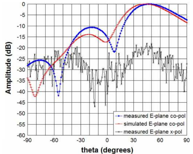
Fig. 8. Measured 2-D radiation patterns of the microstrip quad-Yagi array at 5.2 GHz.
