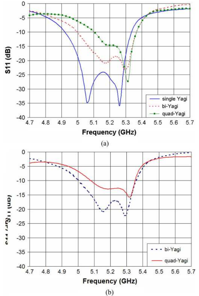
Fig. 5. (a) Simulated return loss of the three Yagi arrays and (b) measured return loss of the designs proposed in this letter.
