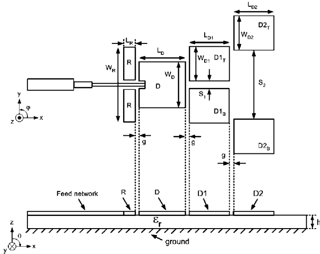
Fig. 3. Illustration of original microstrip Yagi array antenna.
