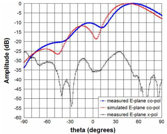
Fig. 7. Measured 2-D radiation pattern of the microstrip bi-Yagi array at 5.2 GHz.
