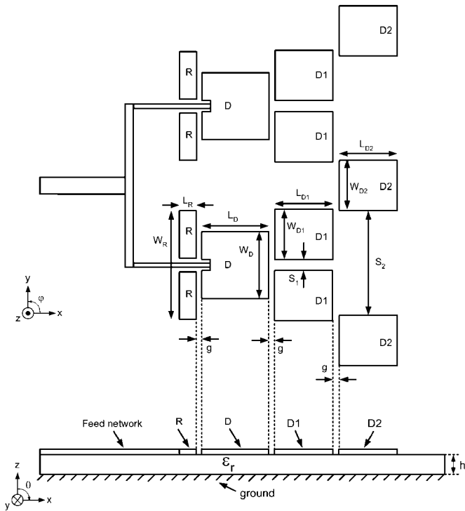
Fig. 1. Illustration of microstrip bi-Yagi array antenna.
