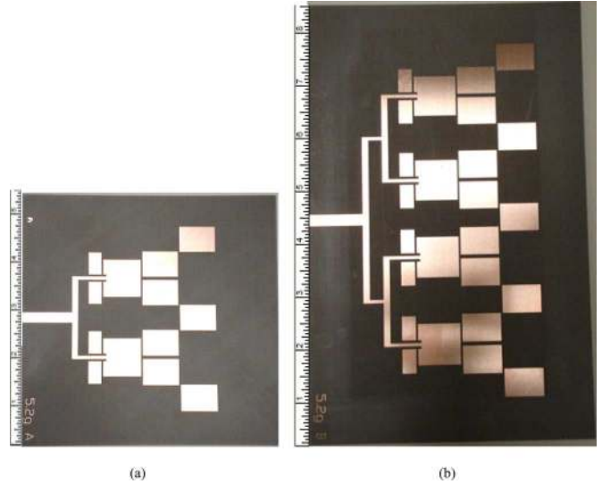
Fig. 4. Illustration of fabricated (a) microstrip bi-Yagi array and (b) microstrip quad-Yagi array antenna. The scales are in inches.
