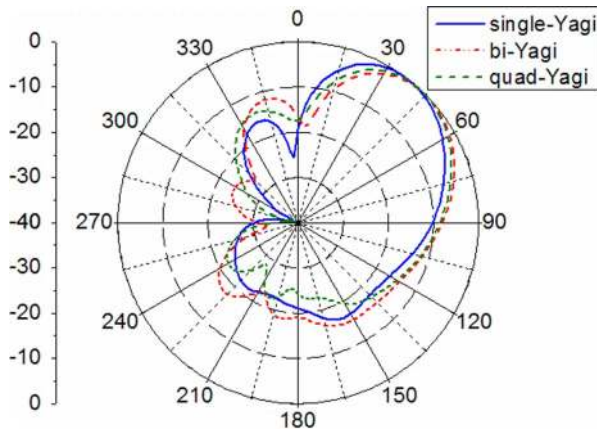
Fig. 6. Simulated 2-D radiation patterns of the three Yagi arrays at 5.2 GHz.
