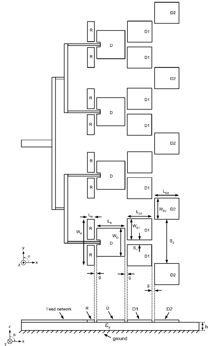
Fig. 2. Illustration of microstrip quad-Yagi array antenna.
