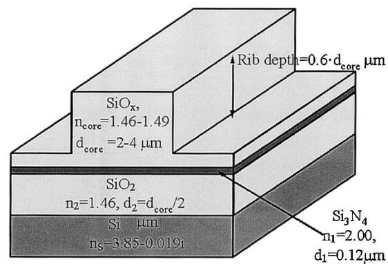
Fig. 2. ARROW structure.
