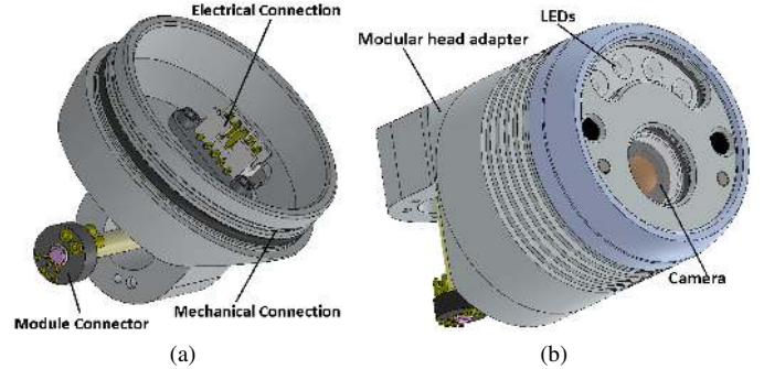
Fig. 8: (a) Modular head adapter and (b) full camera assembly.
