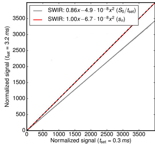
Figure 8. Integration time-normalized signal S_0/t_{\text{set}} (gray line) of the stabilized light source (LIS), measured with the SWIR using two different integration times t_{\text{set}} = 0.3 \text{ ms} and t_{\text{set}} = 3.2 \text{ ms} . The red line shows the signal after normalization ( s_n ) using the corrected integration time t_{\text{set}} + 0.055 \text{ ms} . The dashed line represents the response of a perfectly linear sensor following Eq. (7).
